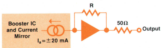
Fig. 1. The Booster IC's current mirror works into the output amplifier's active current sink.
