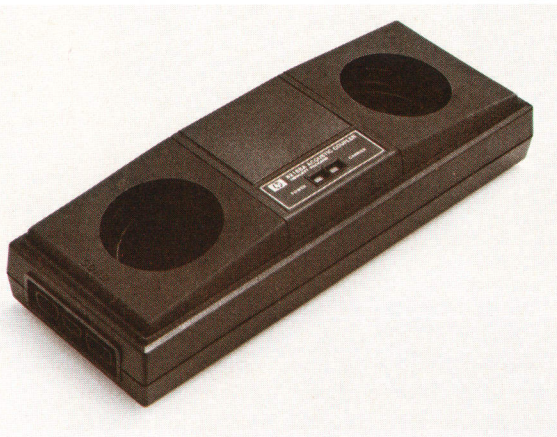
Fig. 1. The HP 82168A Acoustic Coupler can be used to connect any current HP-IL controller such as the HP-75 Portable Computer to a telephone line for transmission of data and programs to another controller or central computer system.
