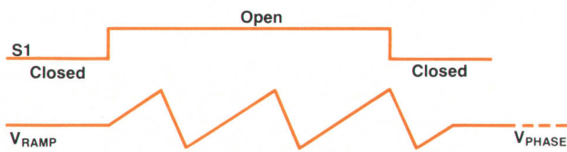
Fig. 8. Snake IC ramp generator timing in triangle mode.
