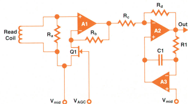
Fig. 10. Analog front-end amplifier circuit.
