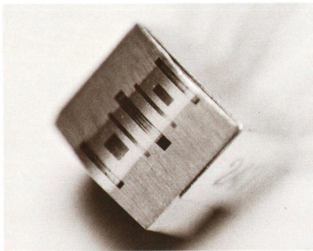
Fig. 3. A common read-after-write head design locates the read and write gaps on opposite sides of the head's crown. The head used in the HP-75 has these gaps located on the crown as shown.
