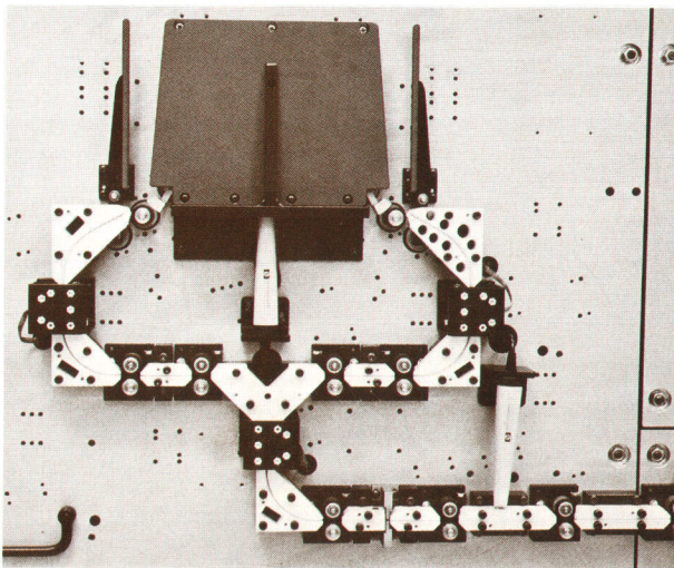
Fig. 2. Card pick module for the production card recorder.
