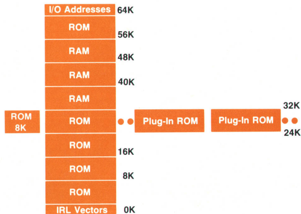
Fig. 3. Memory organization in the HP-75 Portable Computer.
