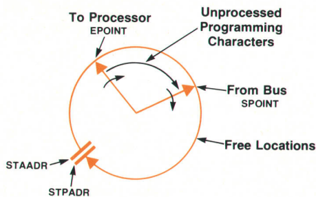
Fig. 6. Structure of the HP-IB buffer in the 8116A and 8112A.
